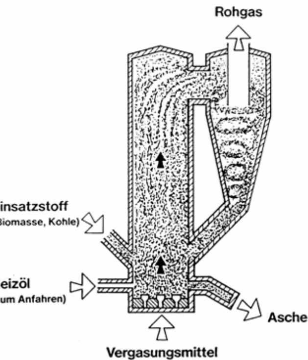
Fluidised Bed (Steam/O 2 )
