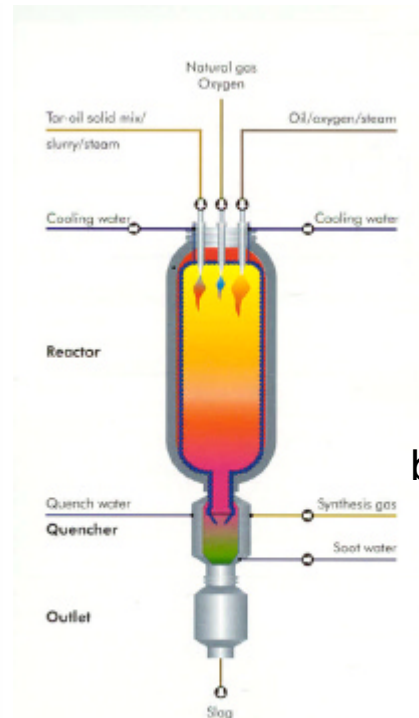
Entrained Flow (O 2 )
