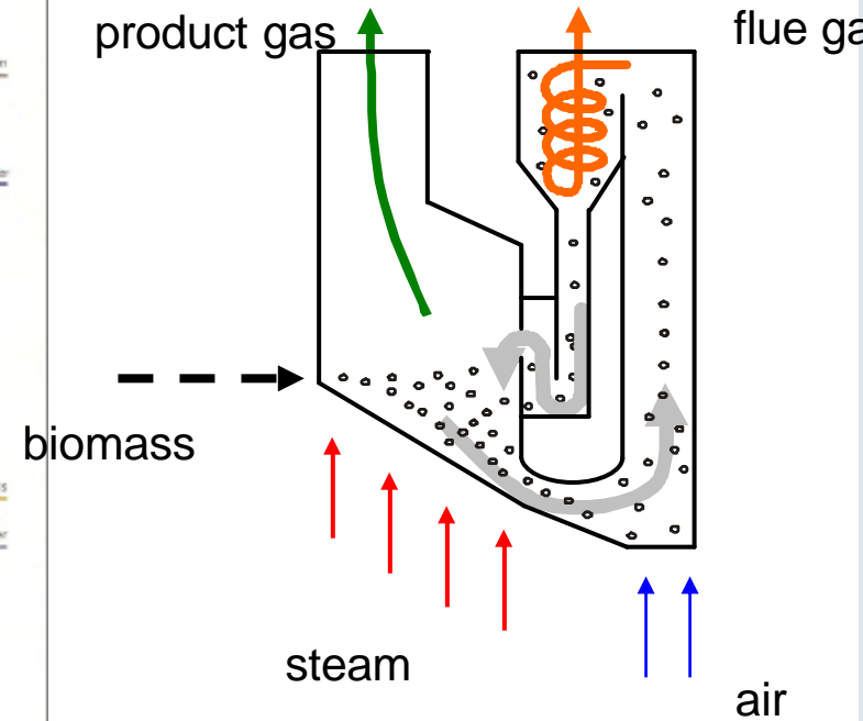
Dual Fluidised Bed (Steam)
