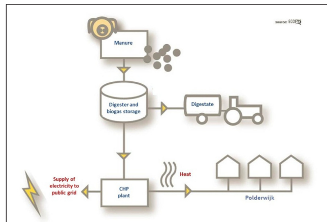
Figure 1. A schematic drawing of the system for biogas production, digestate utilisation, heat and power production and utilisation.
